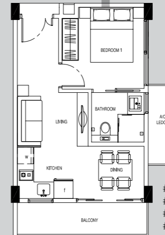
TYPE C (43 sqm)/(463 sq ft)
